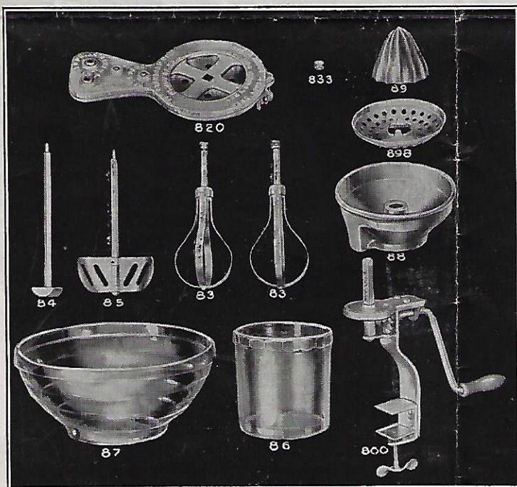
All Parts of No. 82 Dandy Kitchen Machine Unit
